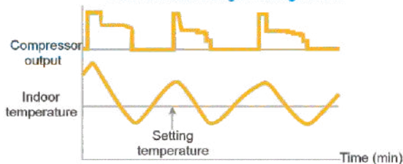
Conventional refrigerant regulation
