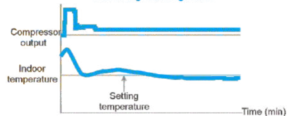
V8S refrigerant regulation
