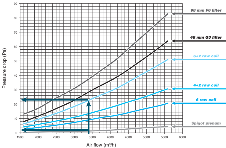
Diagram for Maestro MTL 64 “Available pressure”
