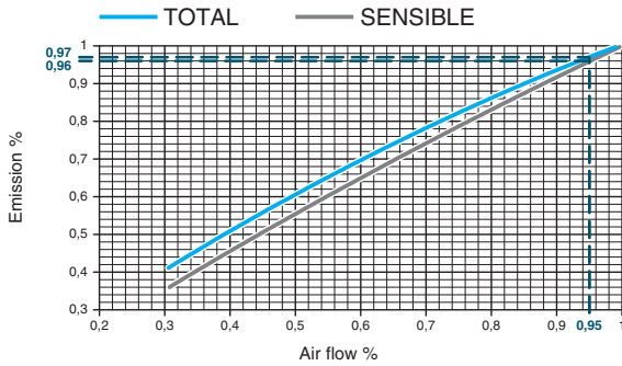
Diagram 2 – Heating emission
