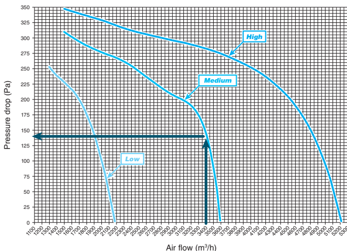
Diagram for Maestro MTL 64 “Available pressure”
